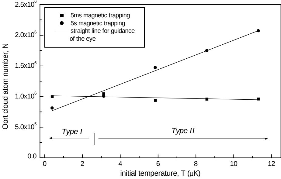
FIGURE 8.7: Atom number of the Oort cloud after 5 s of interaction with a cold cloud for different initial temperature. For low initial temperature a loss in the Oort cloud atom number is observed (Type I). For high initial temperature the Oort cloud atom number increases (Type II).
