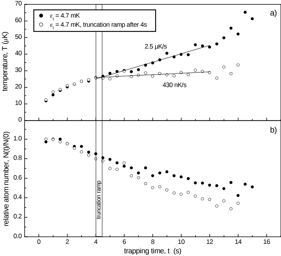
FIGURE 8.3: Temperature a), and atom number b) of a magnetically tapped cloud of initially 2.3 \times 10^7 atoms at 2.7 \mu\text{K} : For a deep trap heating at 2.5 \mu\text{K/s} occurs (solid circles). Ramping down the trap depth at 4s over a period of 0.5s from a truncation energy of 4.7 mK to 420 \mu\text{K} (open circles) heating can be permanently reduced to 0.43 \mu\text{K/s} , whereas no significant change in the atomic loss was found.
