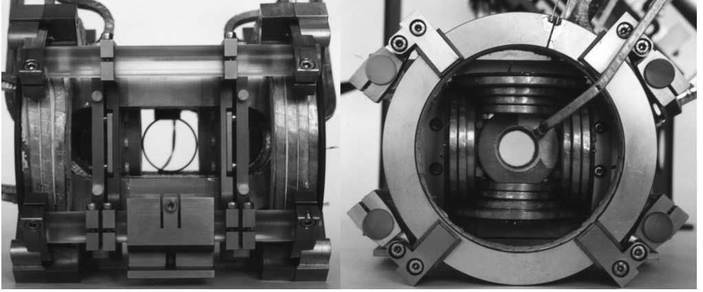
FIGURE 3.3: Ioffe-quadrupole magnetic trap. Left: View along the radial direction. Right: View along the horizontal symmetry axis. The magnetic field coils are made of water cooled copper tubes dissipating 5.4 kW at 400 A. The thermally stable mount is designed like a bench system with four quartz rods.
