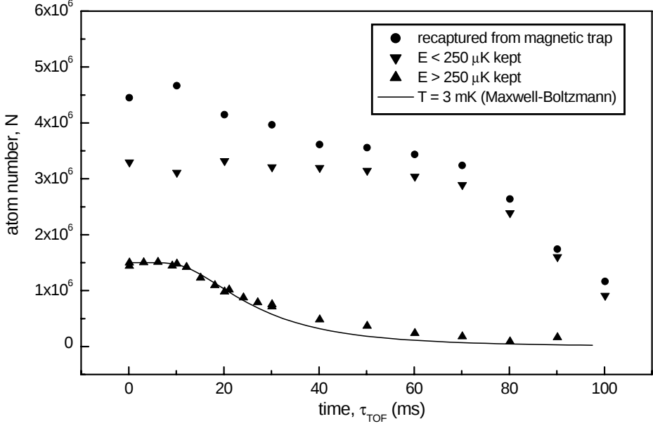
FIGURE 8.4: Time-of-flight measurement of the number of atoms captured after release from the magnetic trap into a MOT. If the full trap contents were recaptured, a bimodal time-of-flight spectrum was measured (circles). Before release from the magnetic trap atoms at energies > 250 \mu\text{K} were spilled out of the trap by an rf-knife and not recaptured (triangles down), resulting in a TOF spectrum of the cold gas cloud with less atoms left at short times. After spilling atoms of energies < \epsilon_t = 250 \mu\text{K} only atoms from the Oort cloud were recaptured (triangles up) vanishing after short times in the TOF spectrum. The calculated TOF spectrum of 3 mK thermal cloud (solid line) is in fair agreement with the observation for the Oort cloud.
